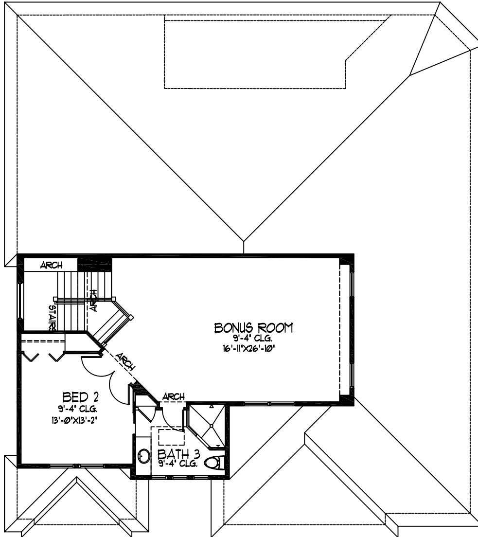
THE SOLANA "A" SECOND FLOOR PLAN
